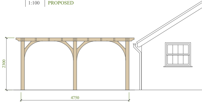
Pergola South Elevation 1:100 PROPOSED
