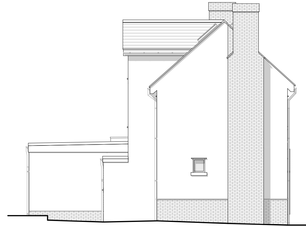
Proposed Side (North) Elevation
