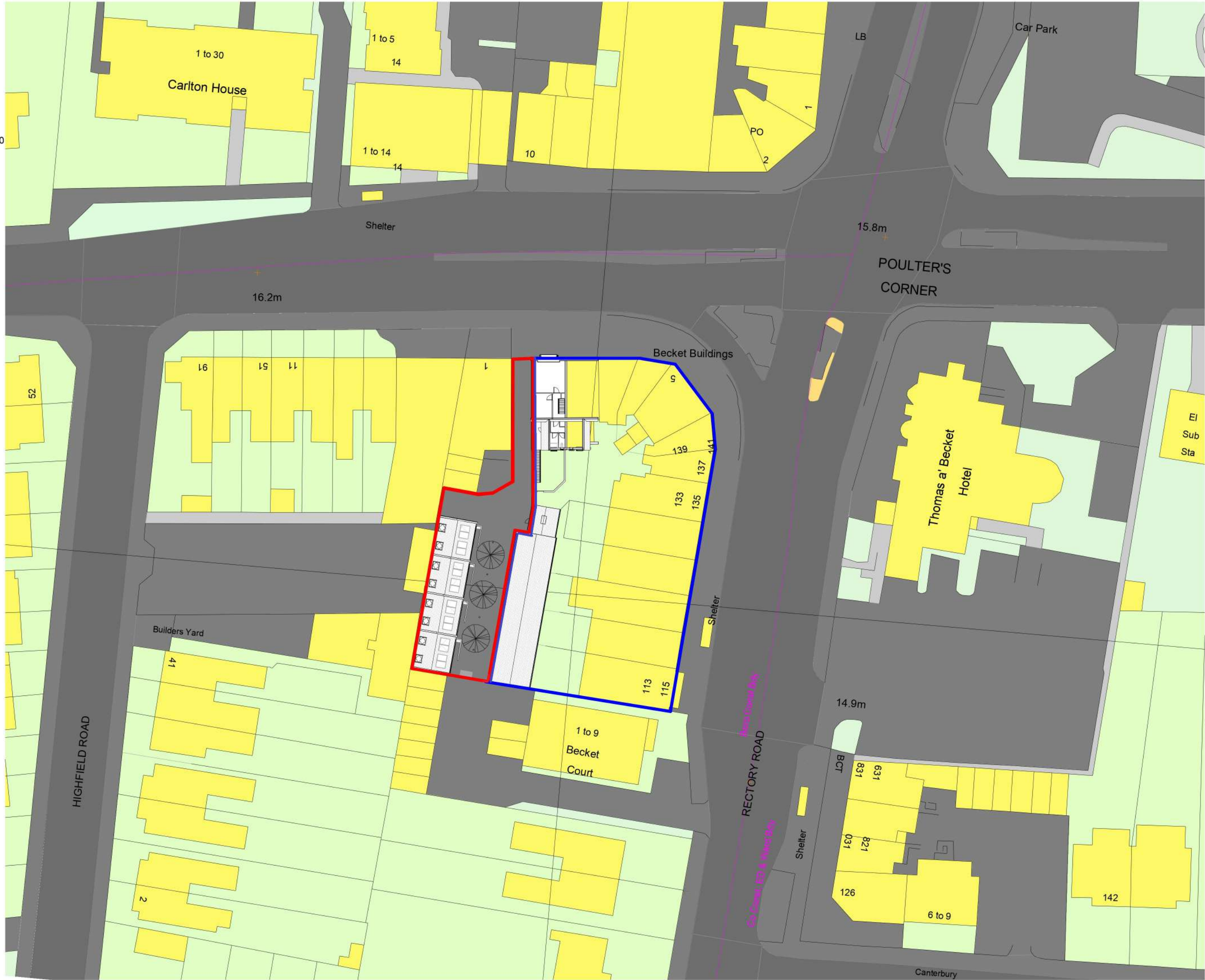
3 Block Plan. 1 : 500 0m 10m 20m 30m 40m 50m VISUAL SCALE 1:500 @ A1
