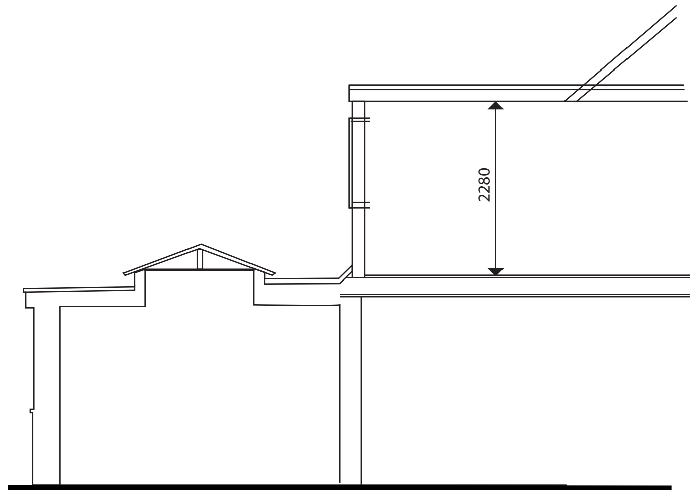
Section A: Proposed new ceiling height for dormer (To match existing) North elevation Scale: 1/50
