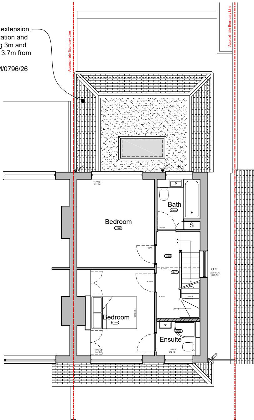
First Floor Plan @ 1:100 Scale
