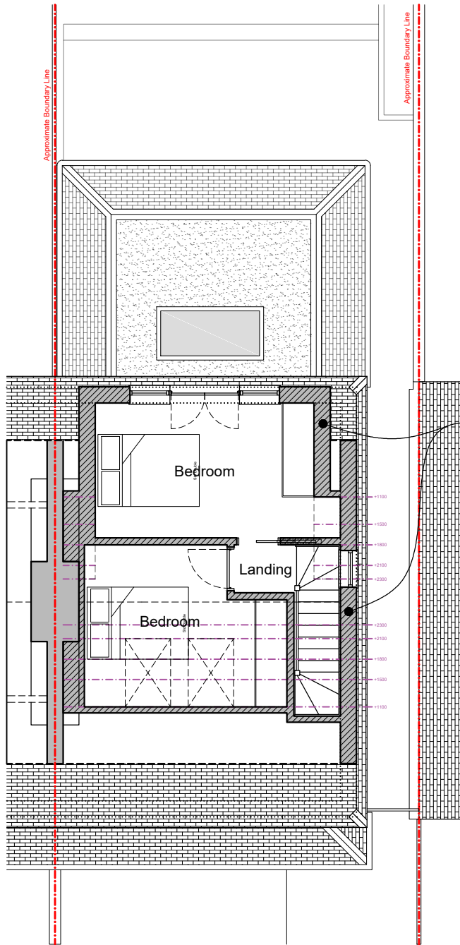
Loft Plan @ 1:100 Scale
