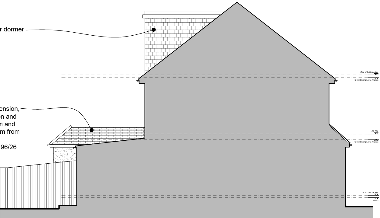
Side (North) Elevation (Through Neighbour) @ 1:100 Scale
