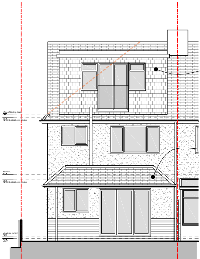
Rear (East) Elevation @ 1:100 Scale
