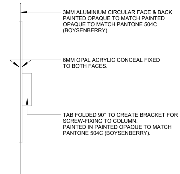
2 NON ILLUMINATED BLADE SIGN - ROUND - DOUBLE SIDED - SECTION 1 : 10
