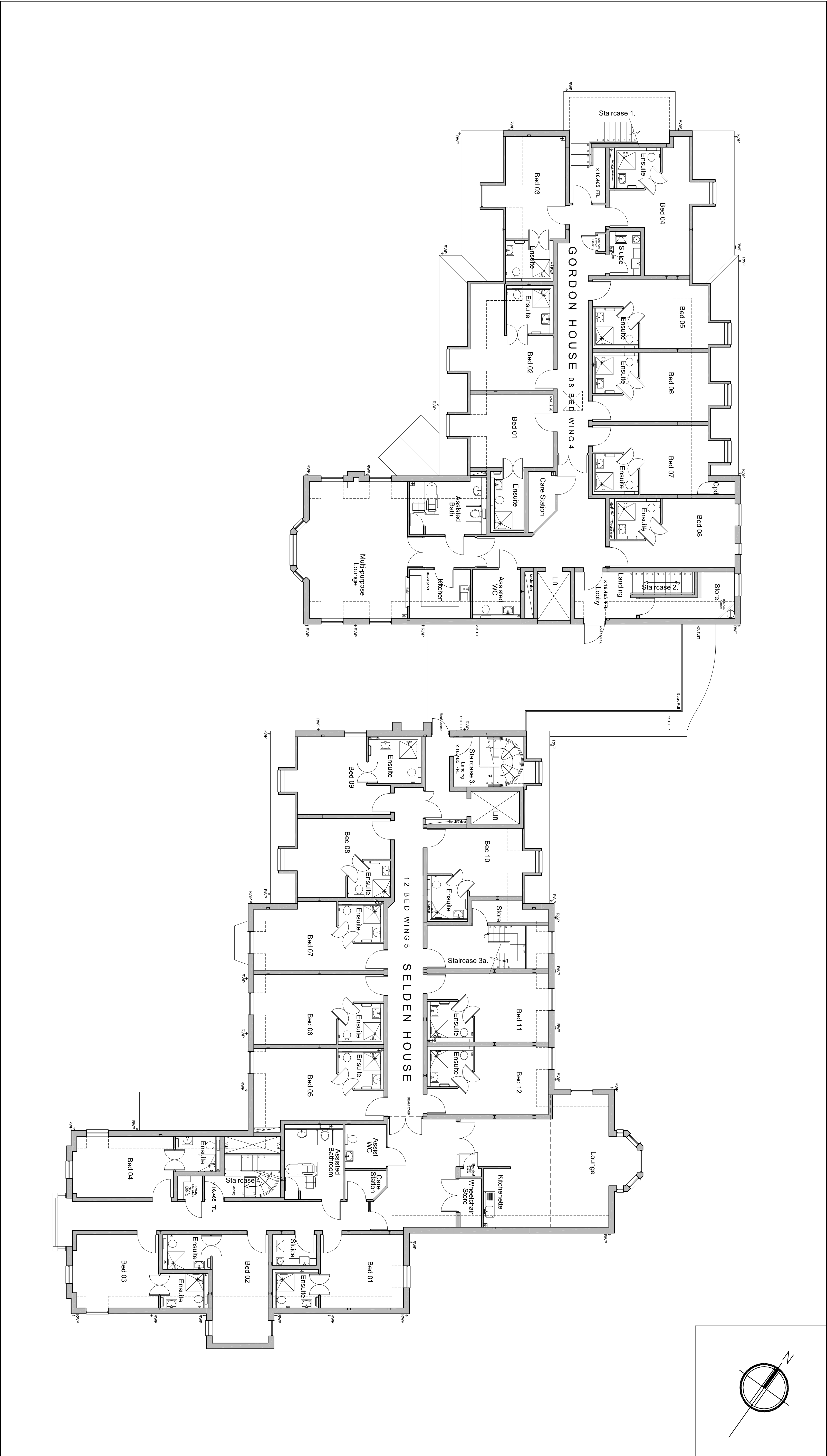
1:100 Second Floor Plan as Existing
