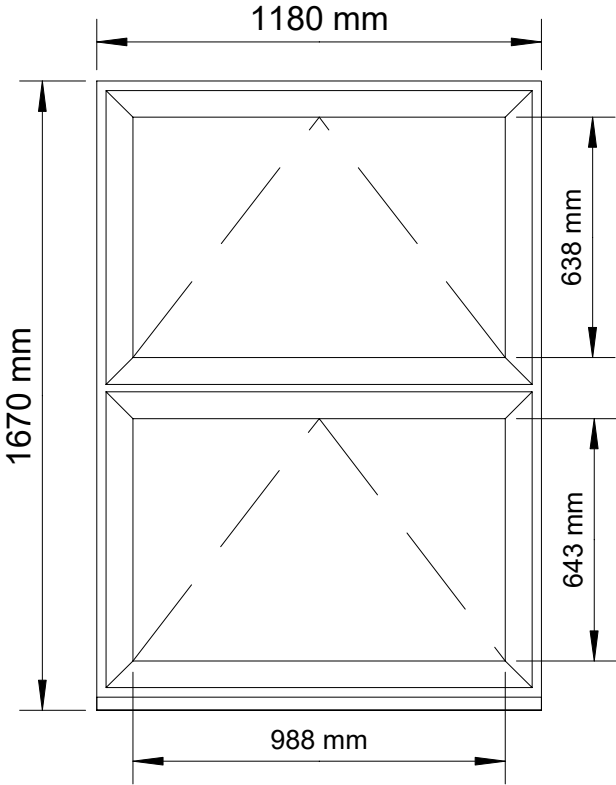
Bedroom Window (Proposed)
