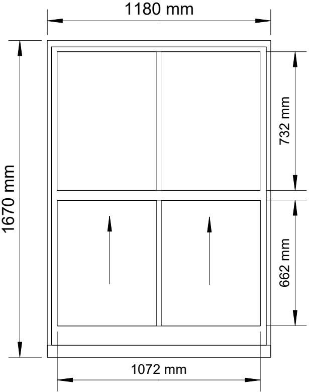
Bedroom Window (Existing)
