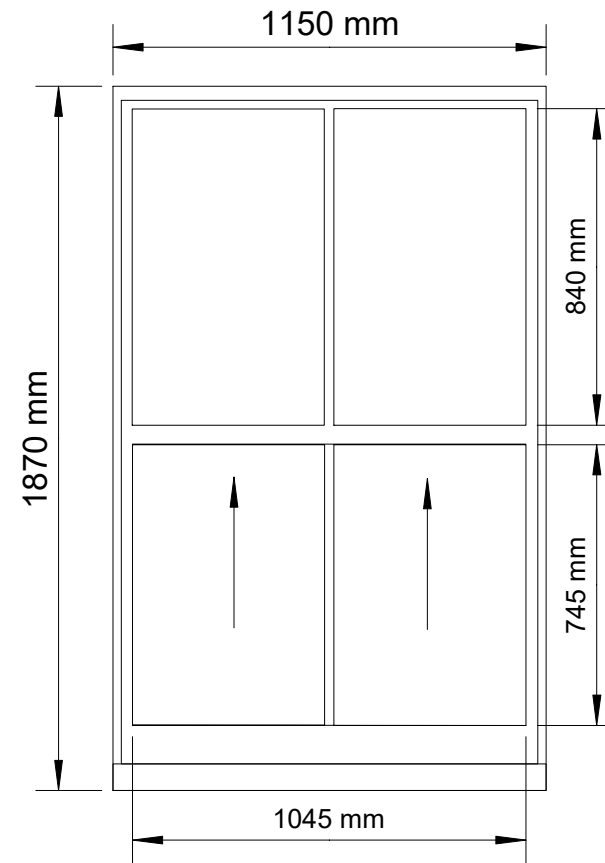
Living Room Window (Existing)
