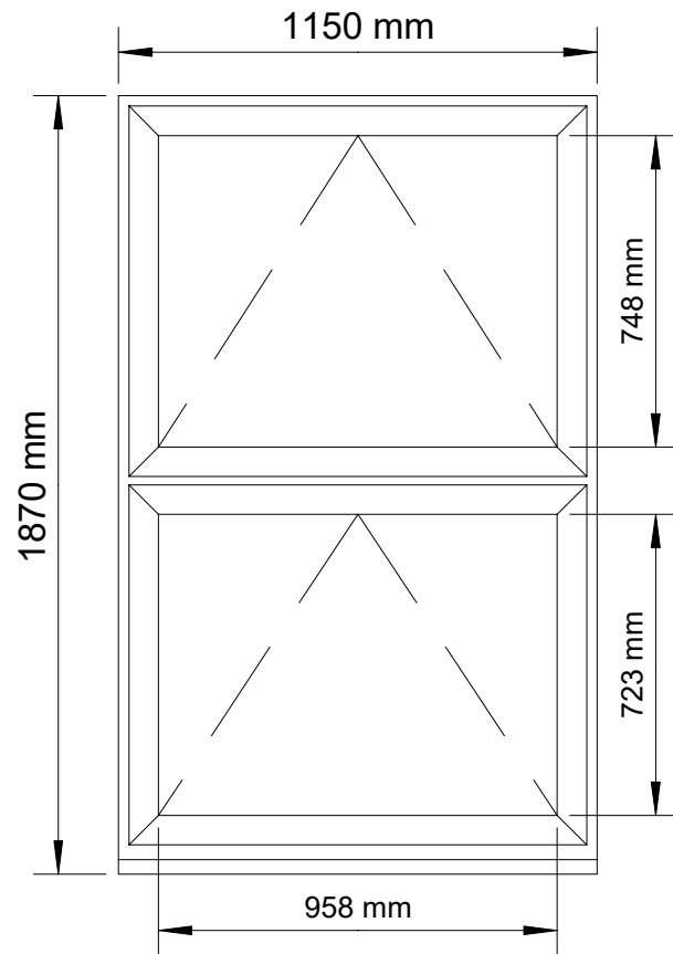
Living Room Window (Proposed)
