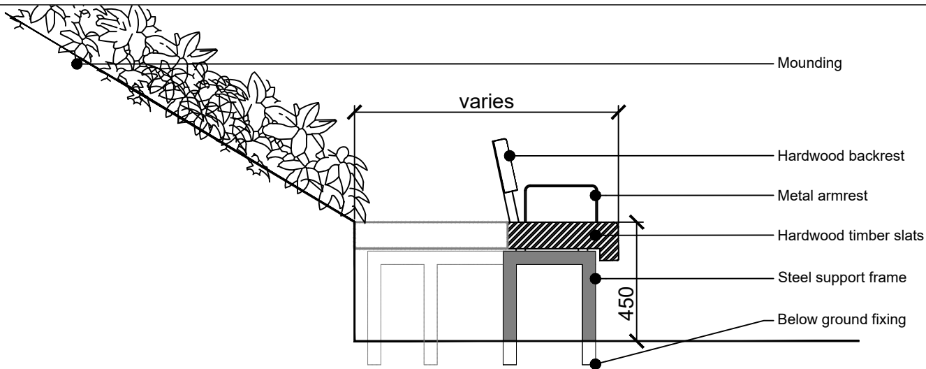
2 SECTION OF BENCH 1:20
