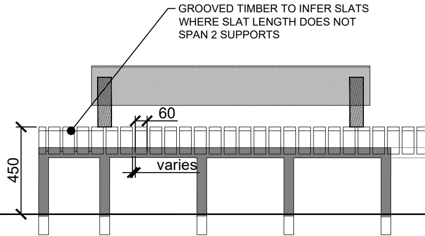
1 ELEVATION OF BENCH 1:20
