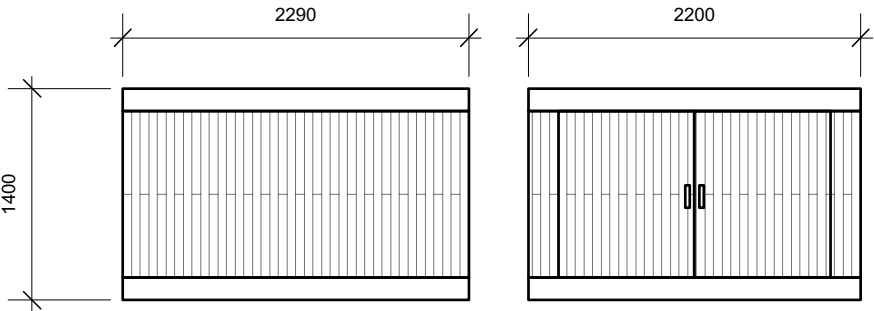
2 Proposed Bike store Scale: 1:50
