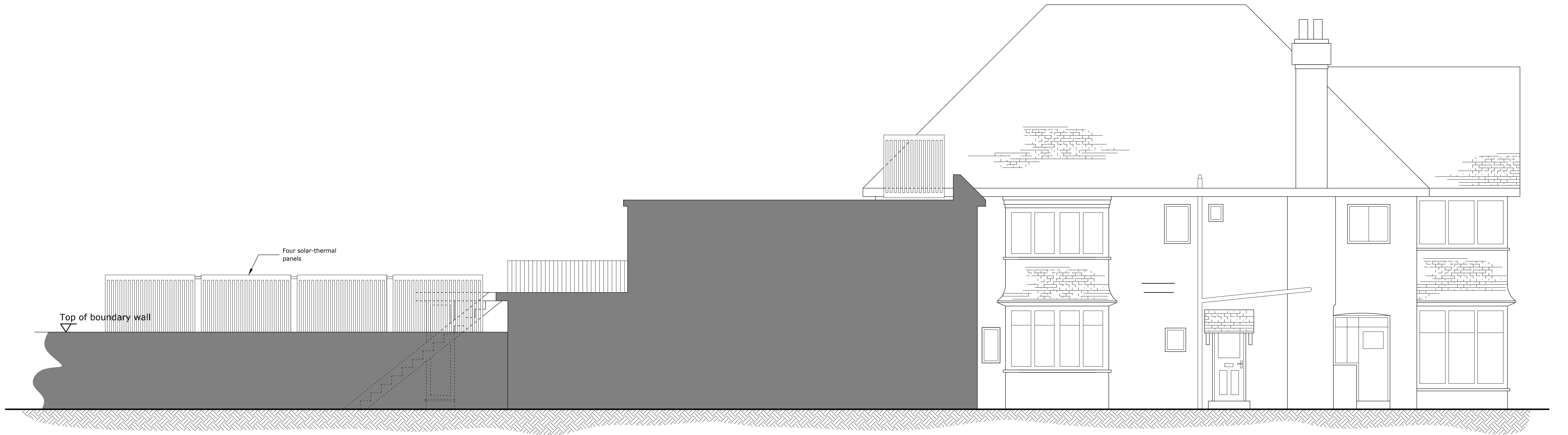
Side (South) Elevation (1:50)
