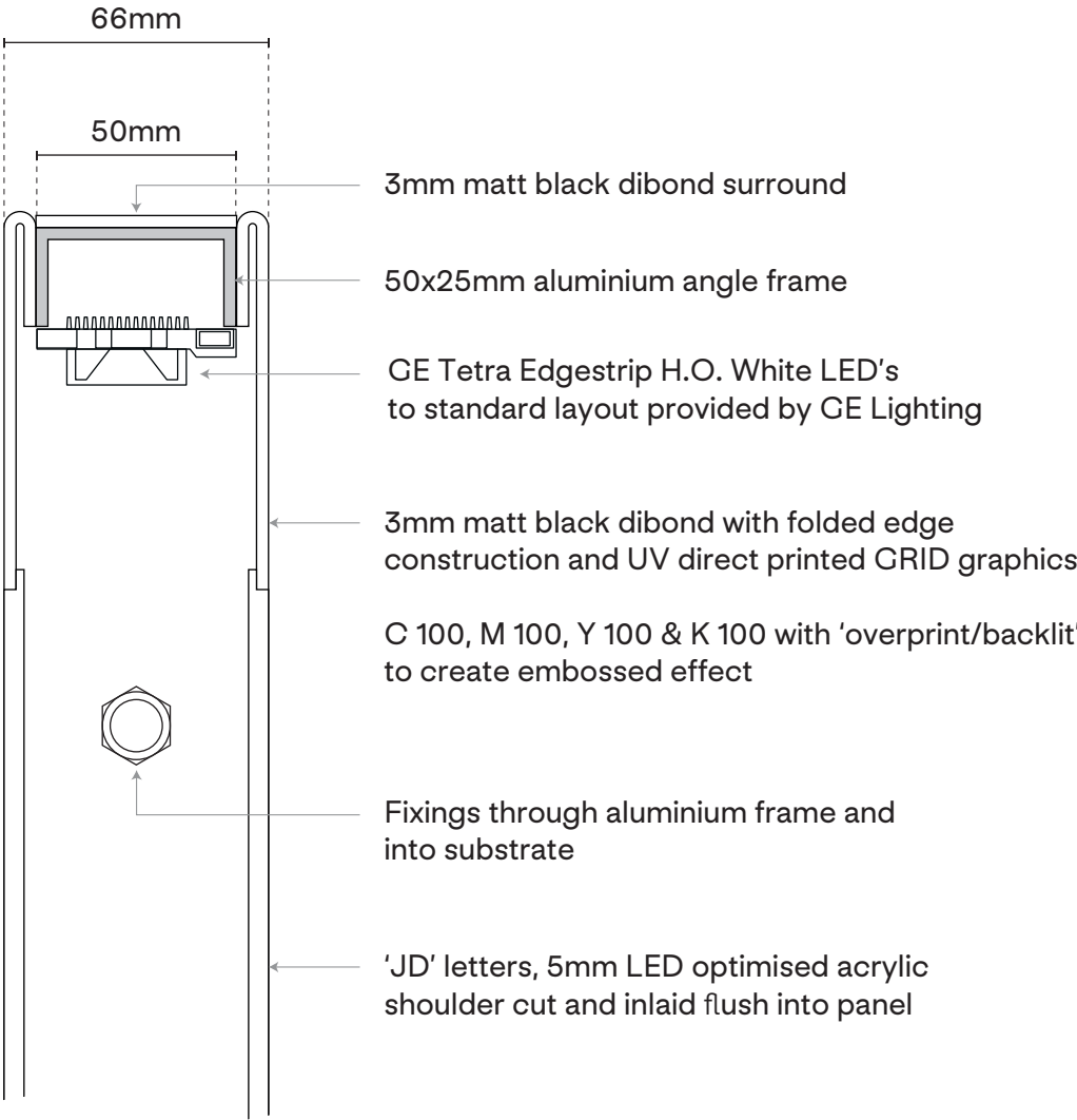
SECTION DETAIL Scale 1:2 @A3
