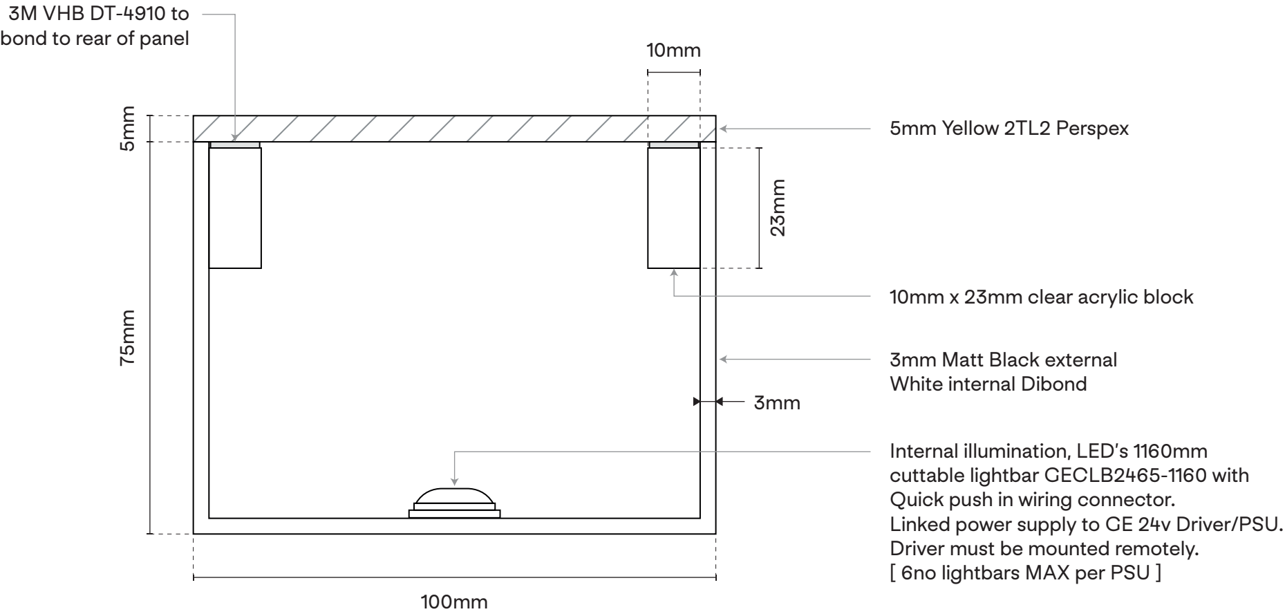
SECTION DETAIL Scale 1:1 @A3
