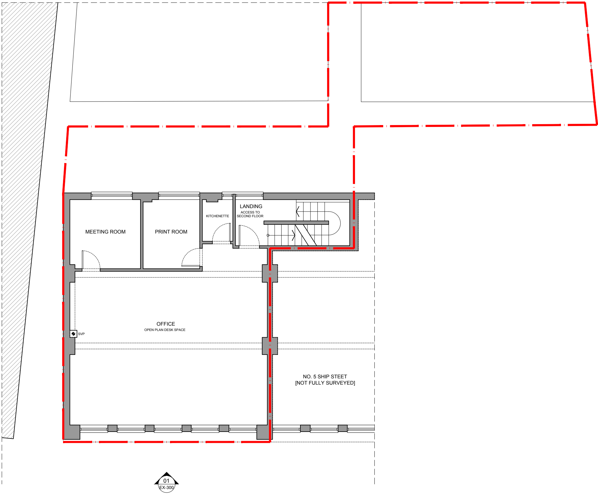
Existing First Floor Plan Scale: 1:100 [A3]
