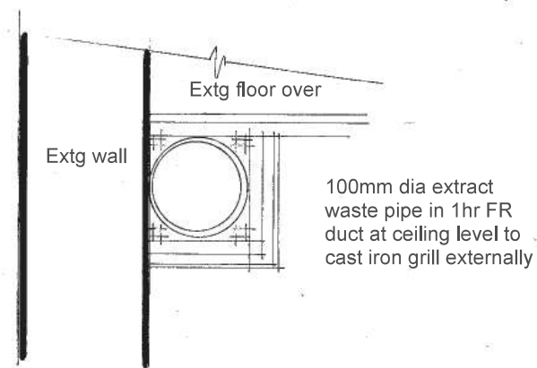
Extract duct detail 1:5
