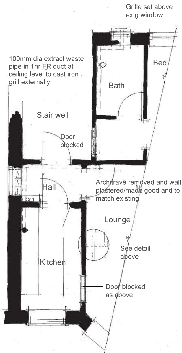
part Plan 1:50
