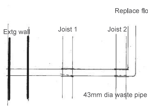
Waste pipe detail 1:10
