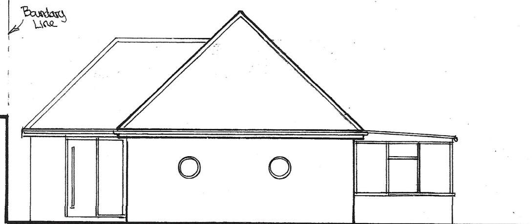
WEST (PRINCIPLE) ELEVATION
