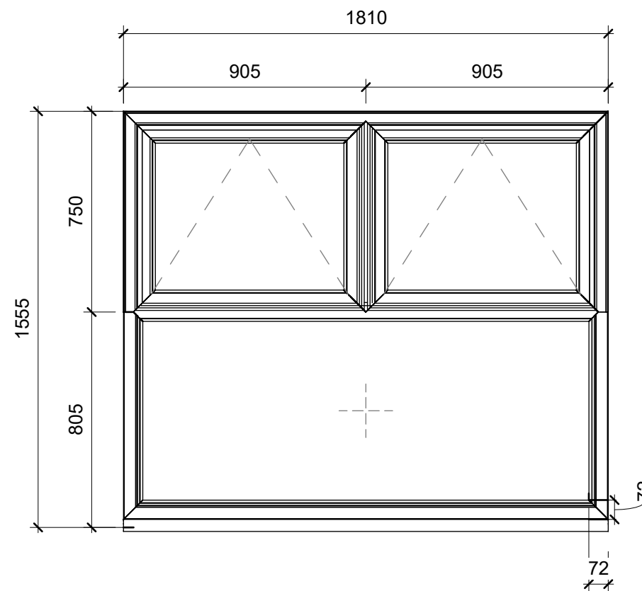
2 Proposed Window Detail 1 : 20
