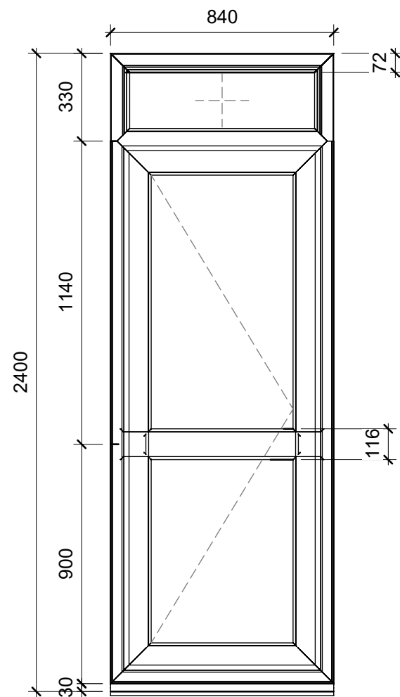
1 Proposed Door Detail 1 : 20
