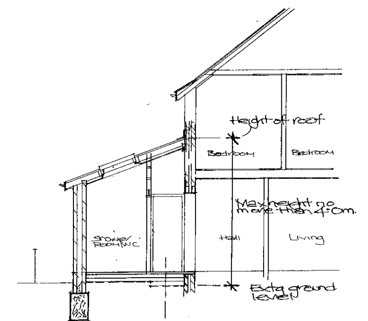
Typical Section - scale: 1/100.
