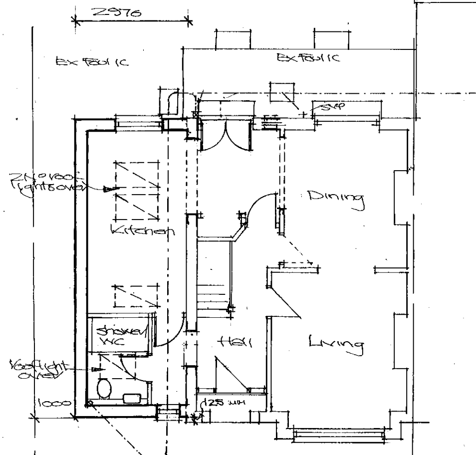
Proposed Ground Floor Scale: 1/100
