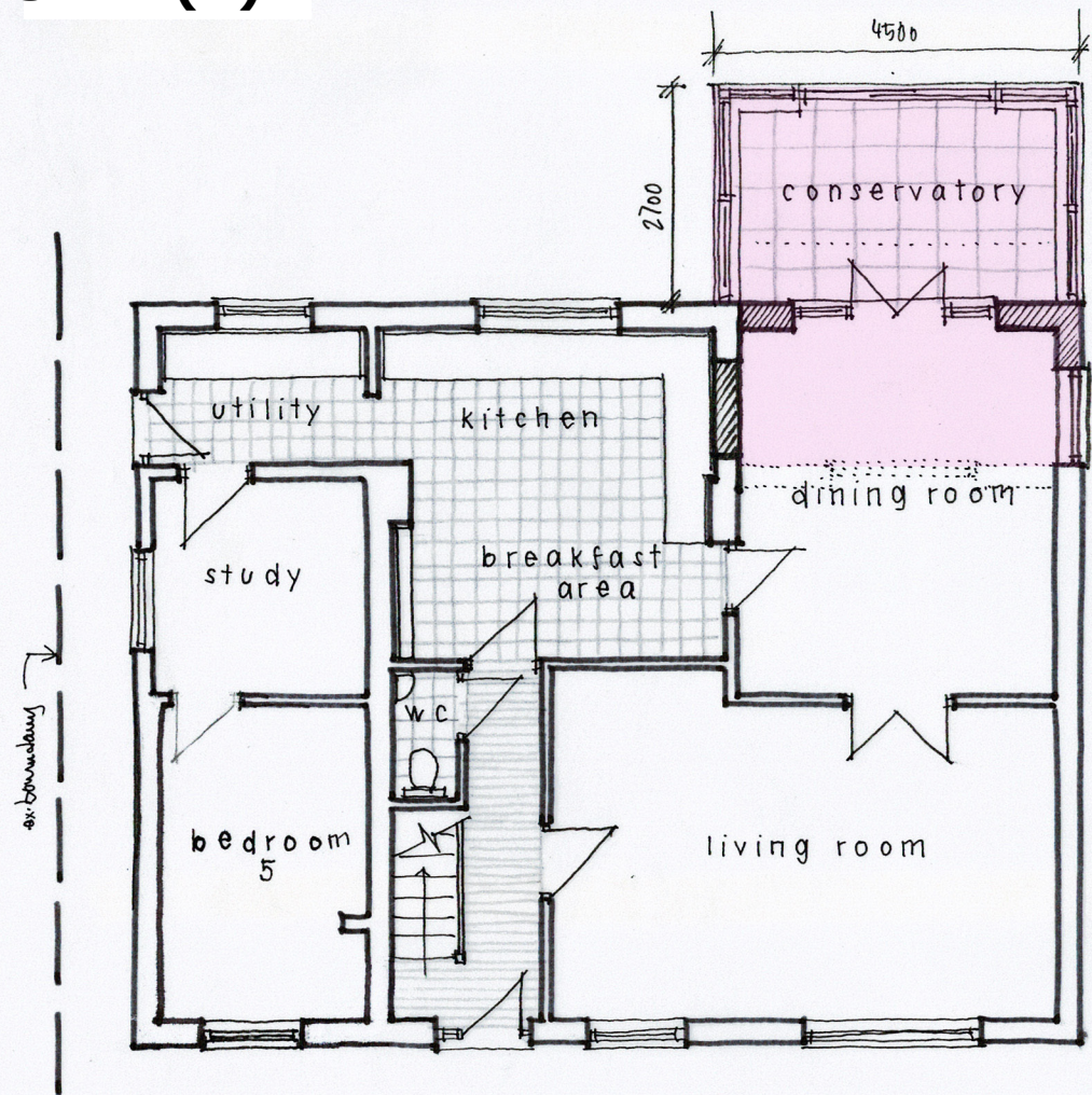
GROUND FLOOR PLAN 1:100 @ A3
