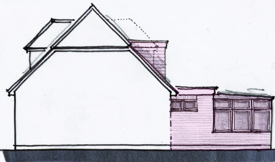
SIDE (s) ELEVATION 1:100 @ A3
