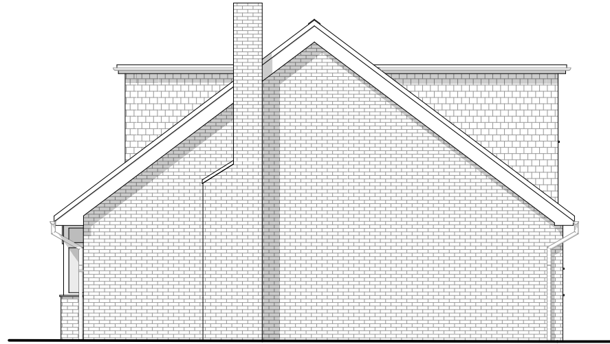
Existing Side (South) Elevation Scale 1:100 @ A3
