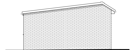
Existing Side (North) Elevation Scale 1:100 @ A3
