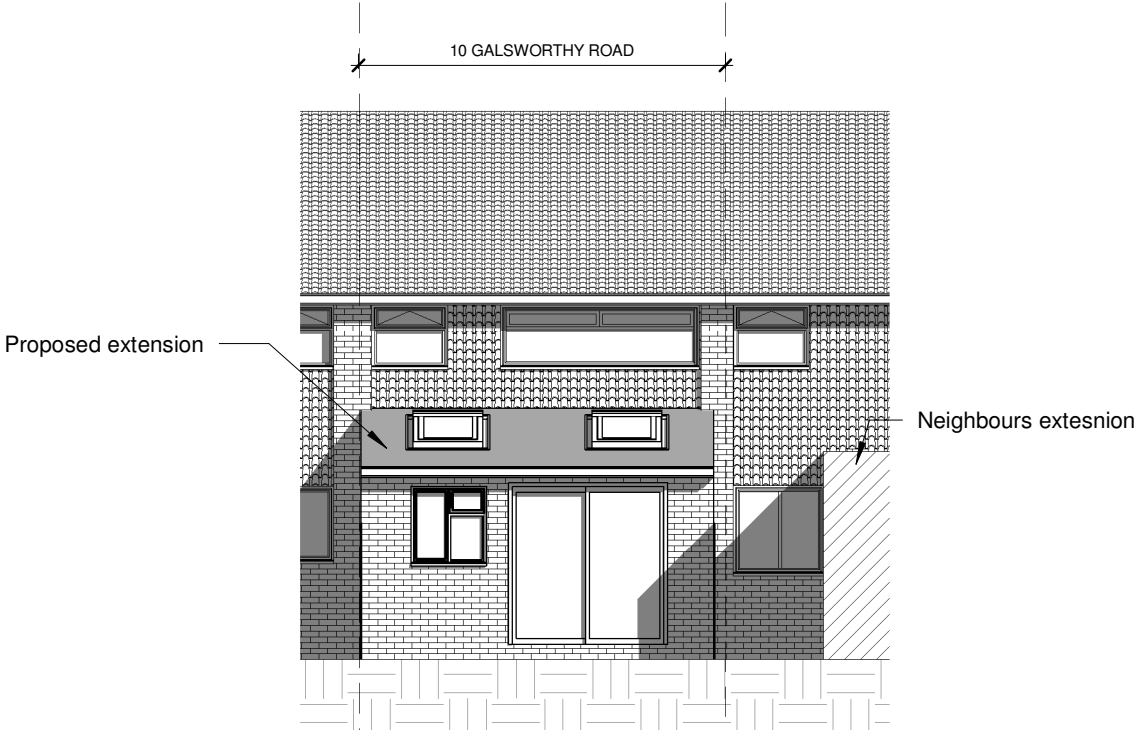
1 ELEVATION FACING WEST 1 : 100
