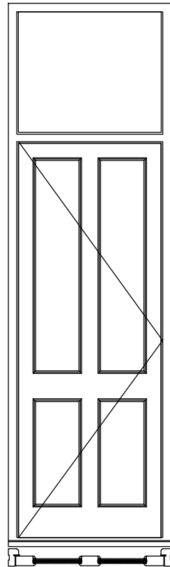
Item 1 Proposed Elevation & Section Drawings Scale 1:20 @ A3
