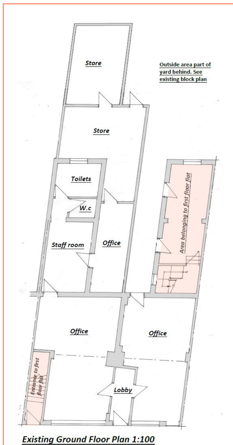
Figure 3: Existing ground floor plan (Source: Applicant)
