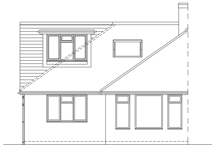
North Elevation
