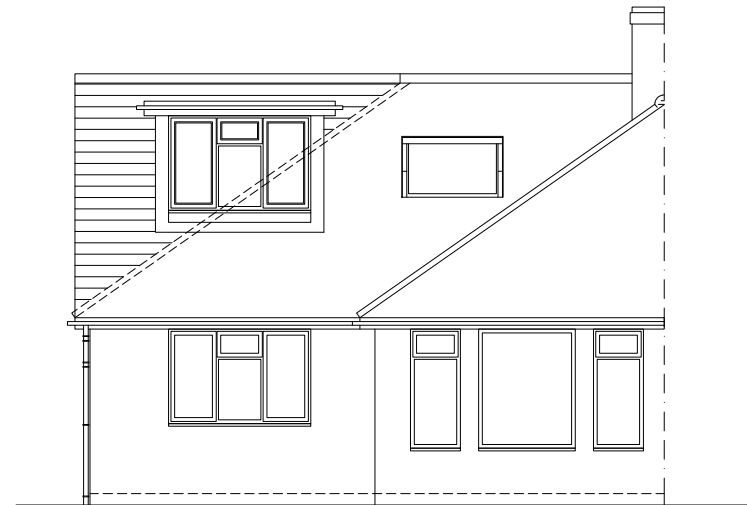
North Elevation
