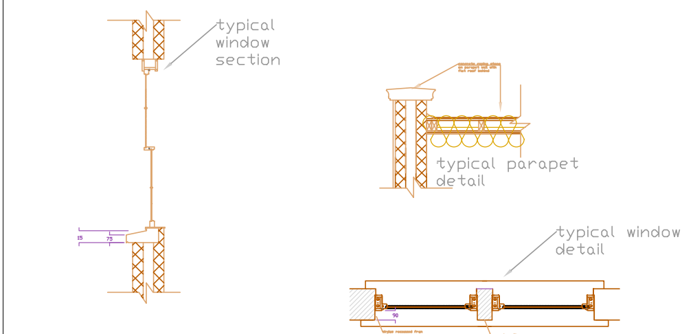
DETAILS 1:50
