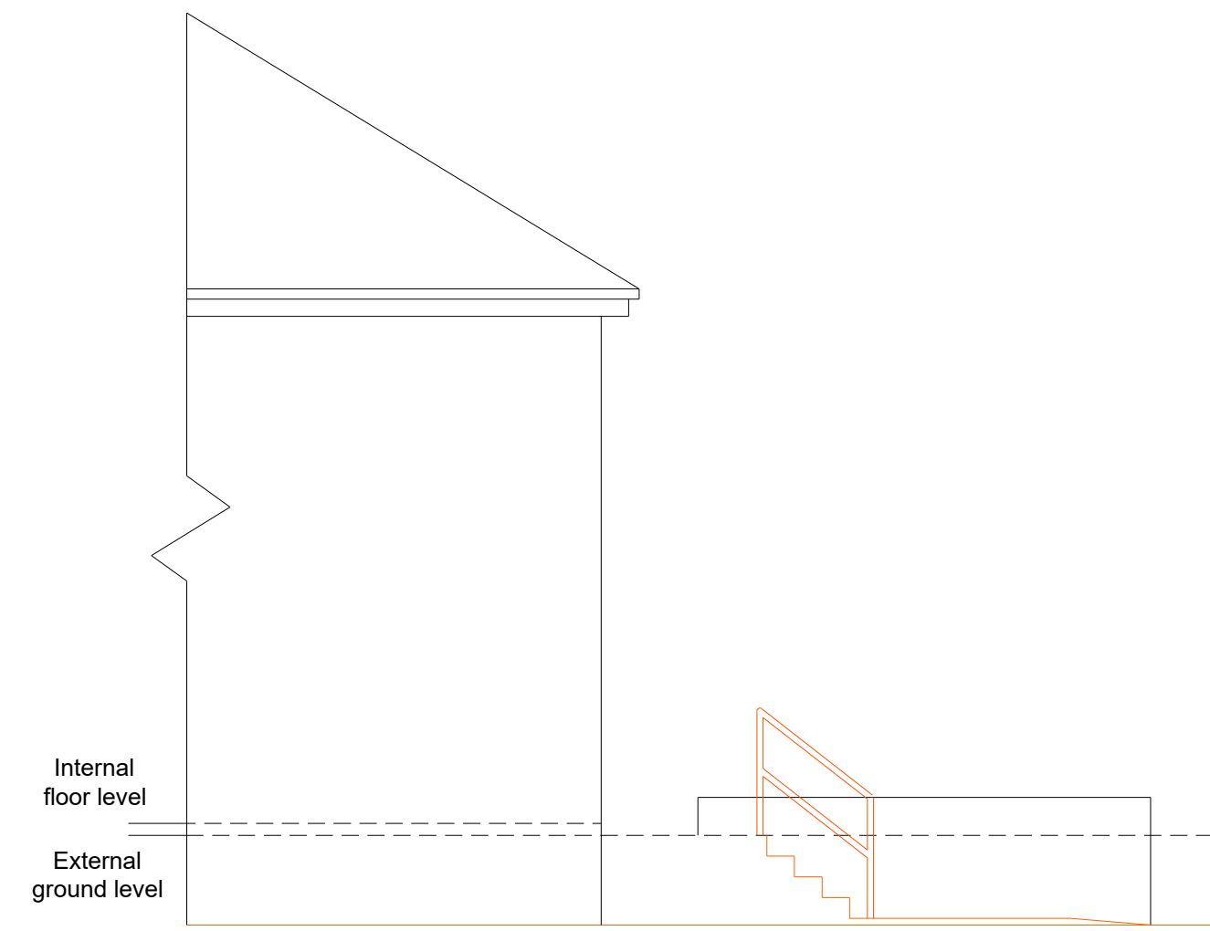
West Elevation - Proposed
