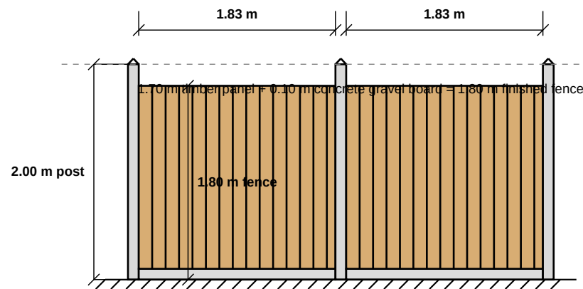
TYPICAL 1.8 m HIGH FENCE ELEVATION
