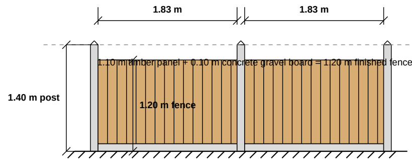
TYPICAL 1.2 m HIGH FENCE ELEVATION
