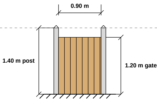
1.2 m HIGH GATE ELEVATION
