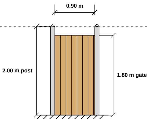
1.8 m HIGH GATE ELEVATION
