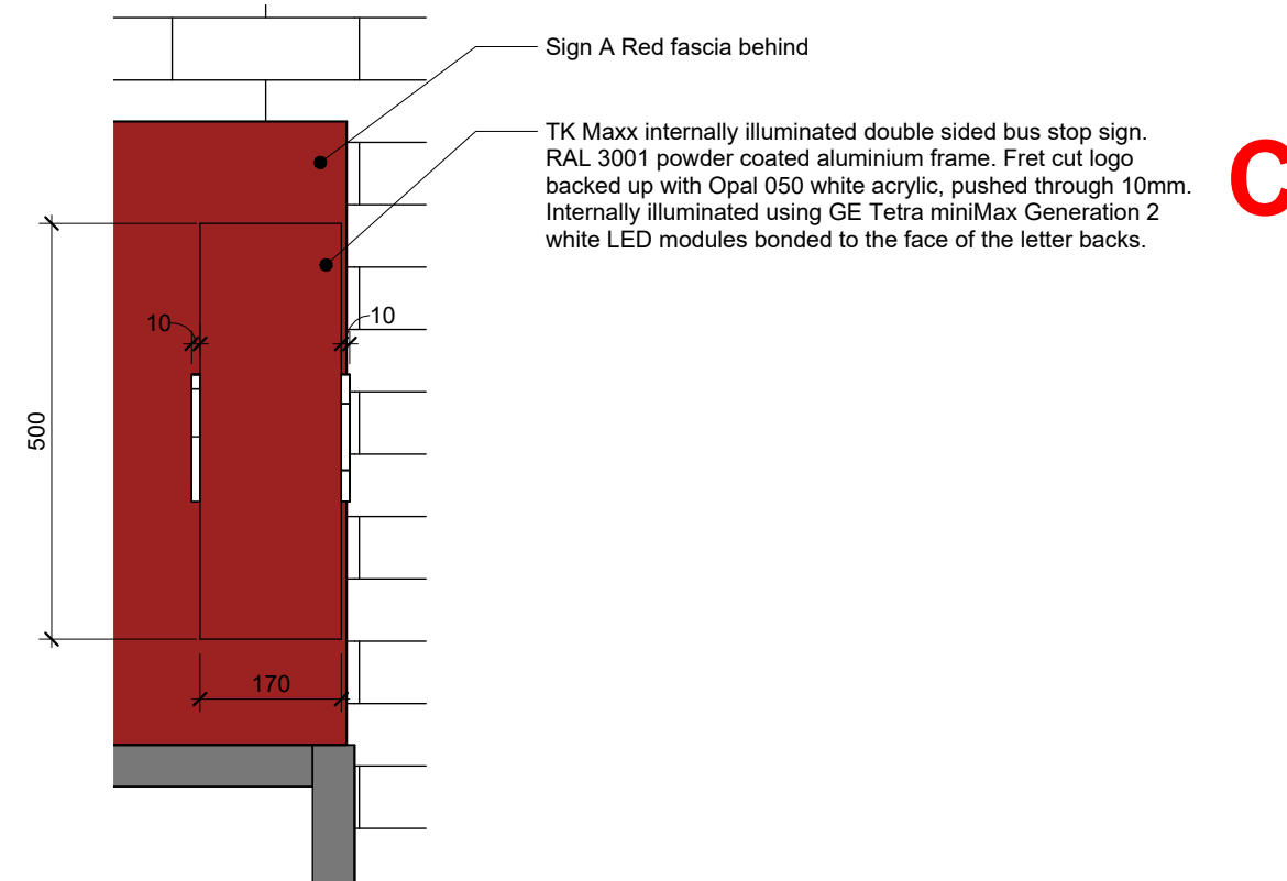
5 SCALE 1 : 10 Section through advert 'C'
