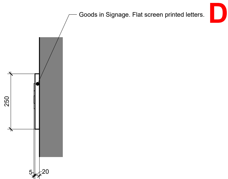
6 SCALE 1 : 10 Section through advert 'D'
