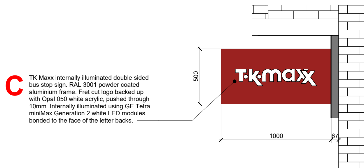
2 SCALE 1 : 20 Advert 'C' - Elevation
