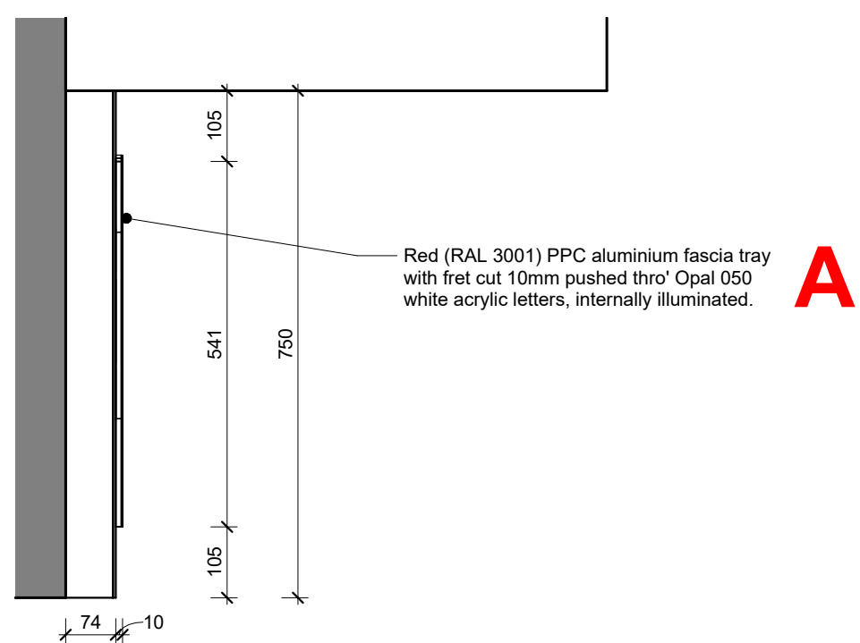
4 SCALE 1 : 10 Section through advert 'A'
