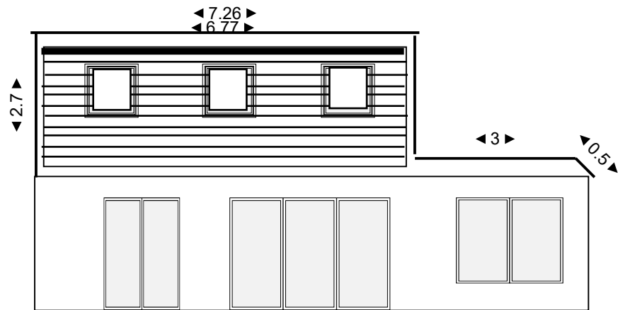
North Elevation
