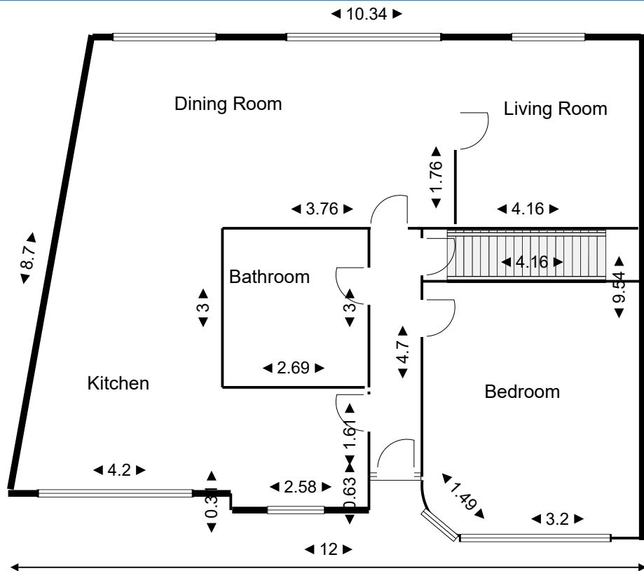
Groundfloor Floor Plan
