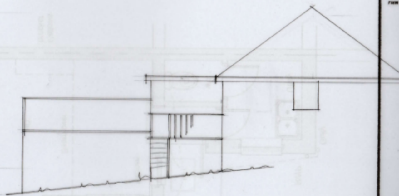
SIDE ELEVATION:-EAST
