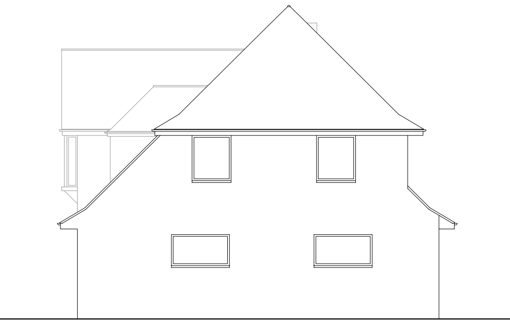
SIDE ELEVATION 1:100
