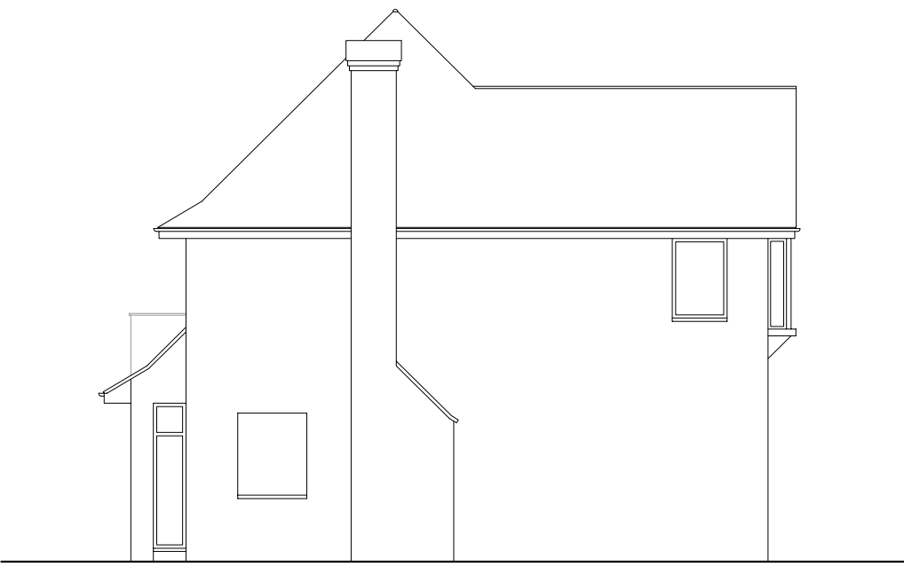
SIDE ELEVATION 1:100
