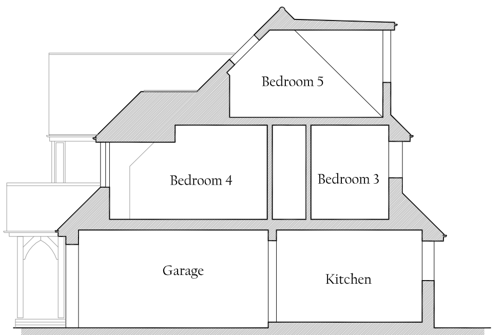
SECTION 1:100
