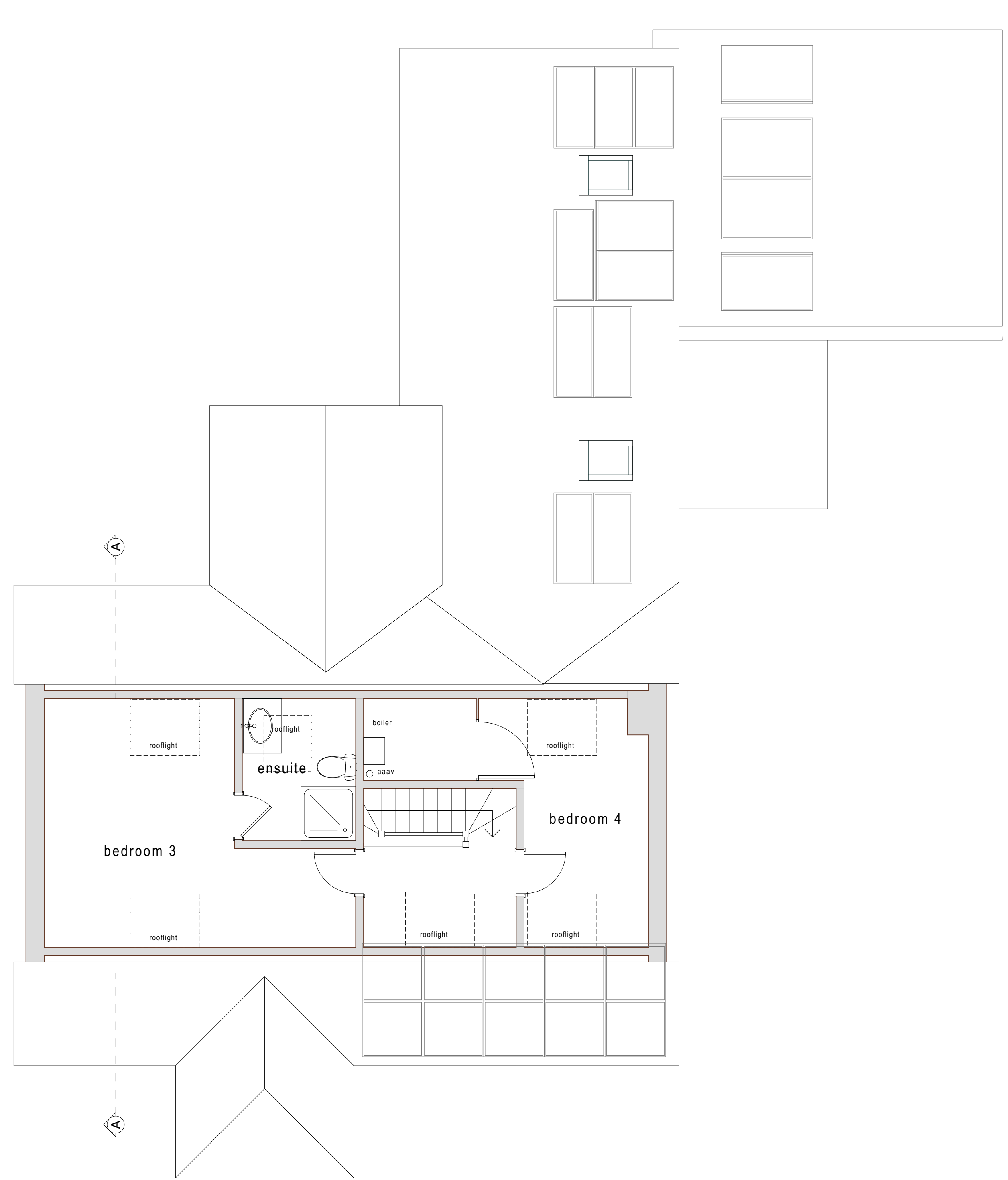
FIRST FLOOR
