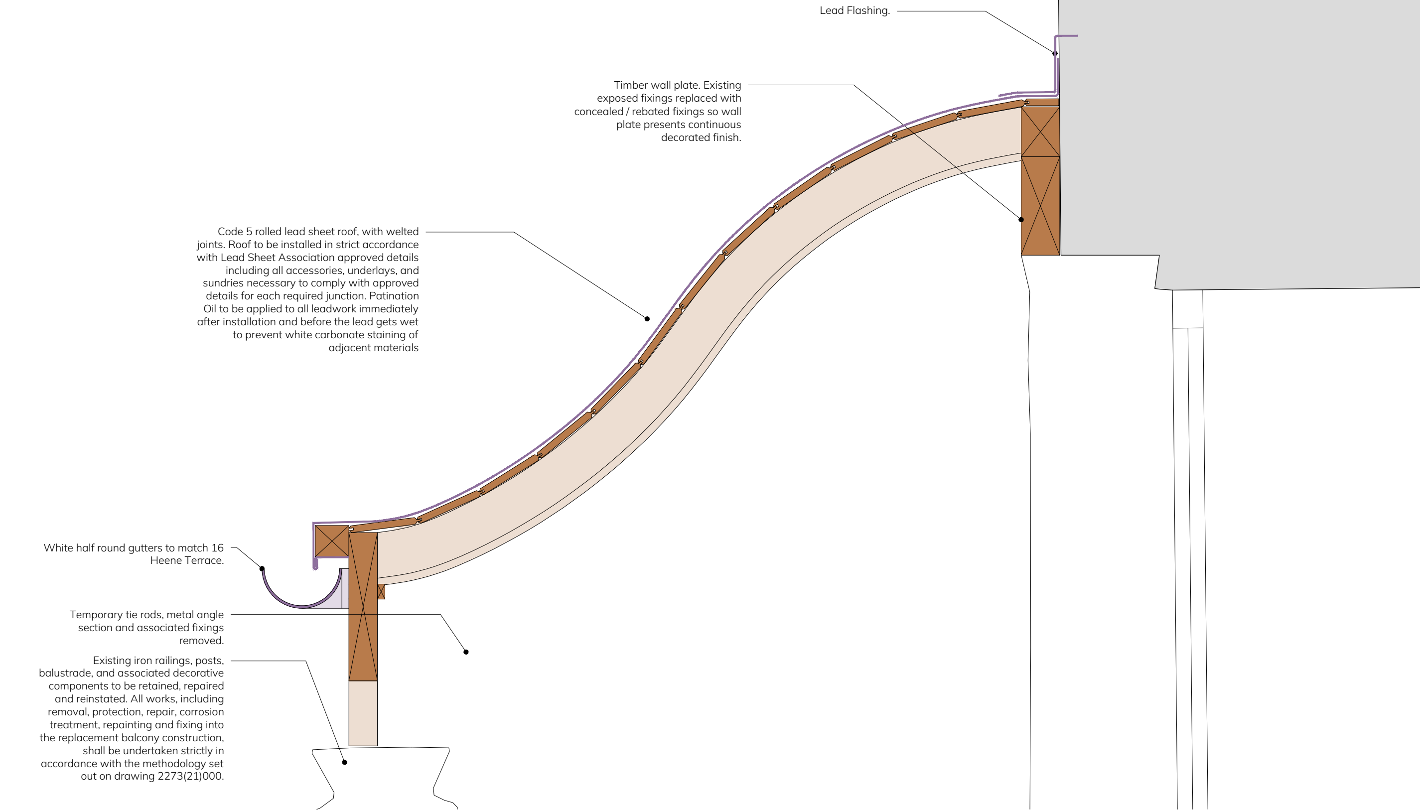
01-As Existing 1:5 Balcony Canopy Detail Section
