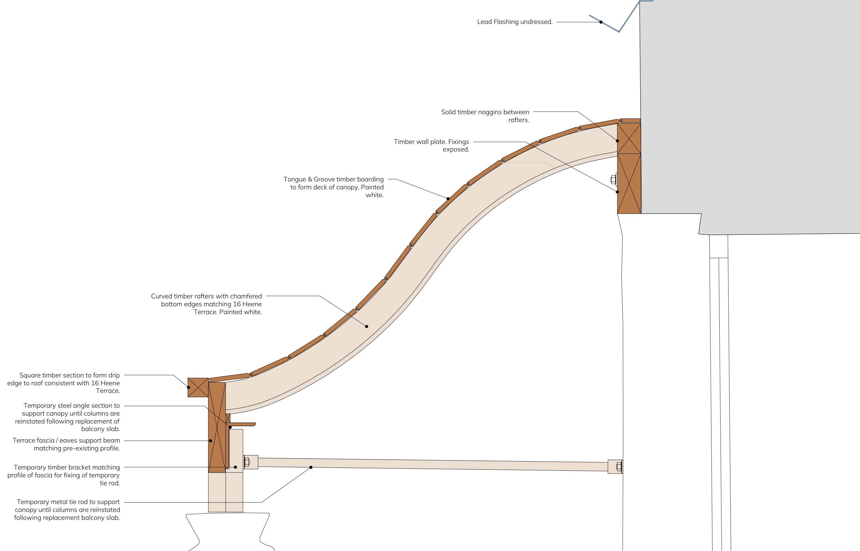
01-As Existing 1:5 Balcony Canopy Detail Section
