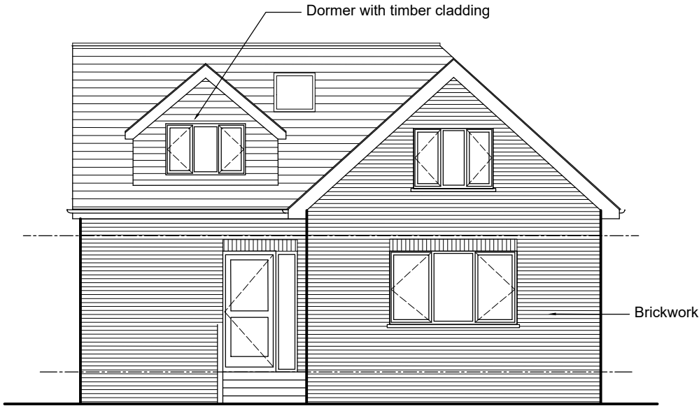
West Elevation
