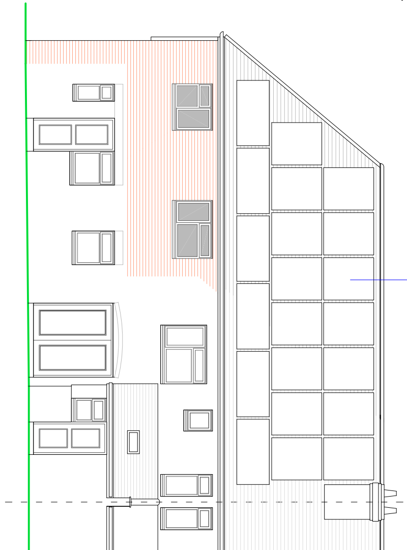
REAR (SOUTH WEST) ELEVATION
