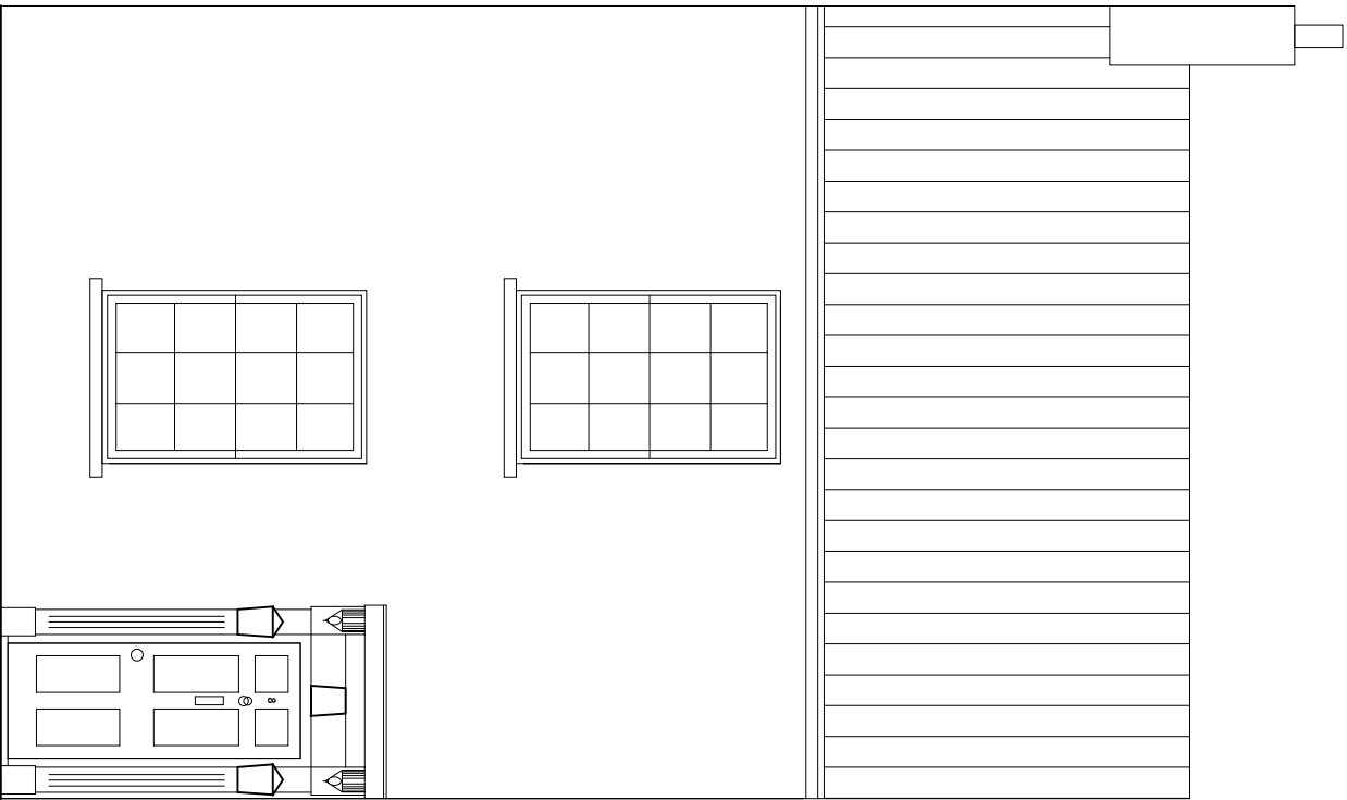
WEST ELEVATION AS EXISTING
