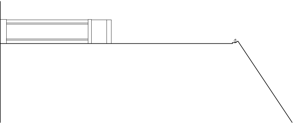
SIDE ELEVATION AS PROPOSED
