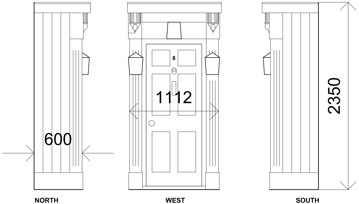
PORCH ELEVATIONS AS EXISTING
