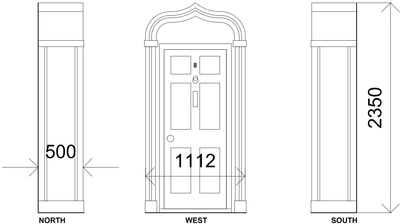
PORCH ELEVATIONS AS PROPOSED
