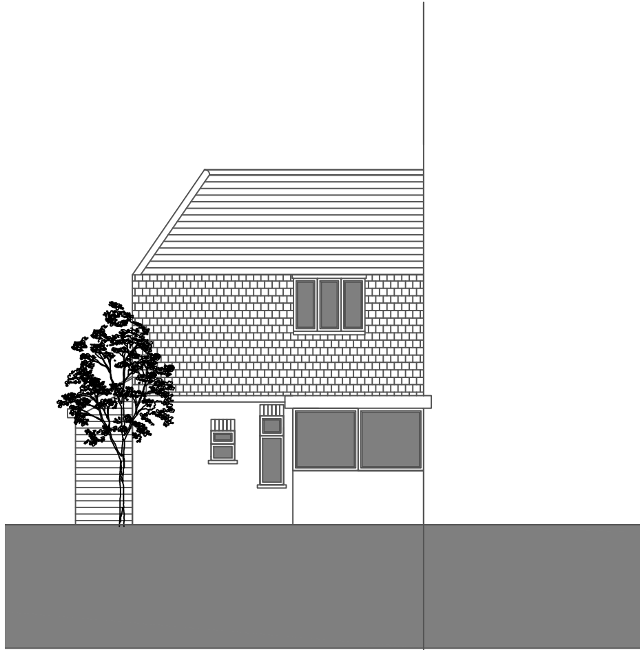
EXISTING NORTH ELEVATION 1:100 @ A3
