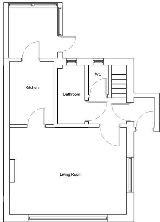
EXISTING FLOOR PLAN 1:100 @ A3
