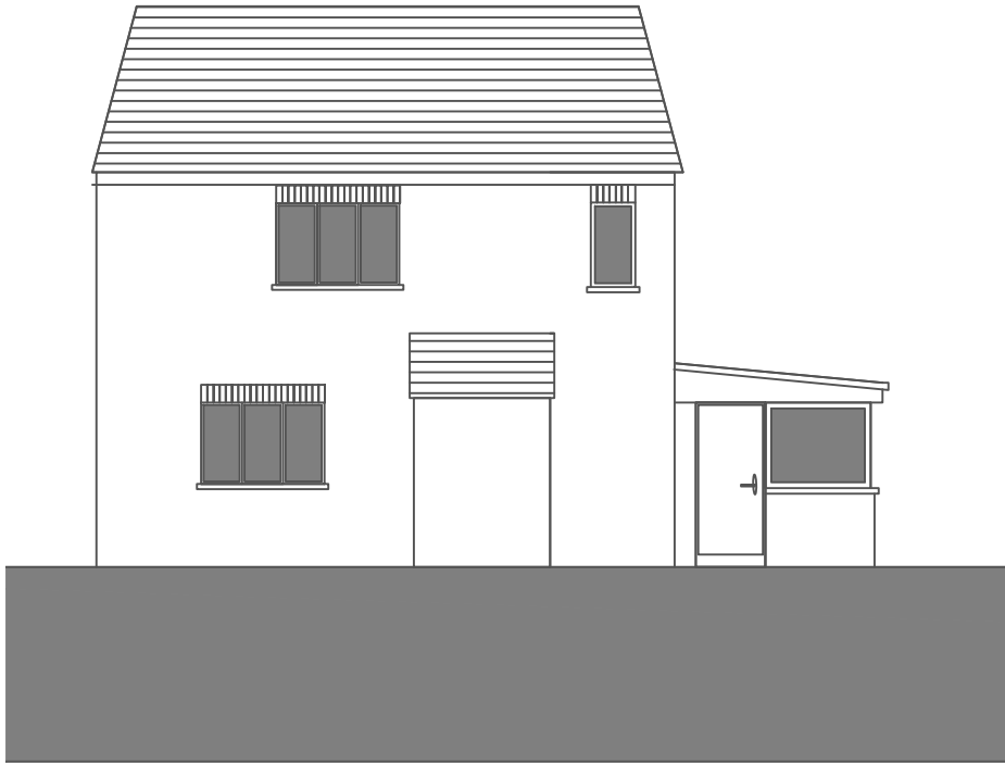
EXISTING EAST ELEVATION 1:100 @ A3
