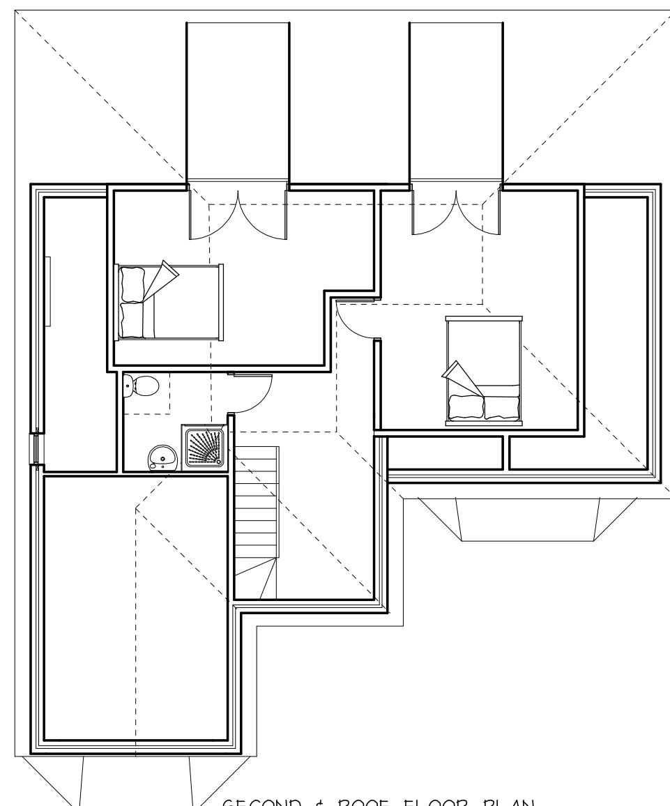
SECOND & ROOF FLOOR PLAN PROPOSED
