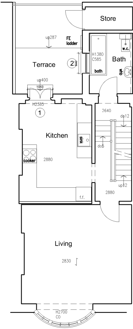
First Floor Plan as Existing
