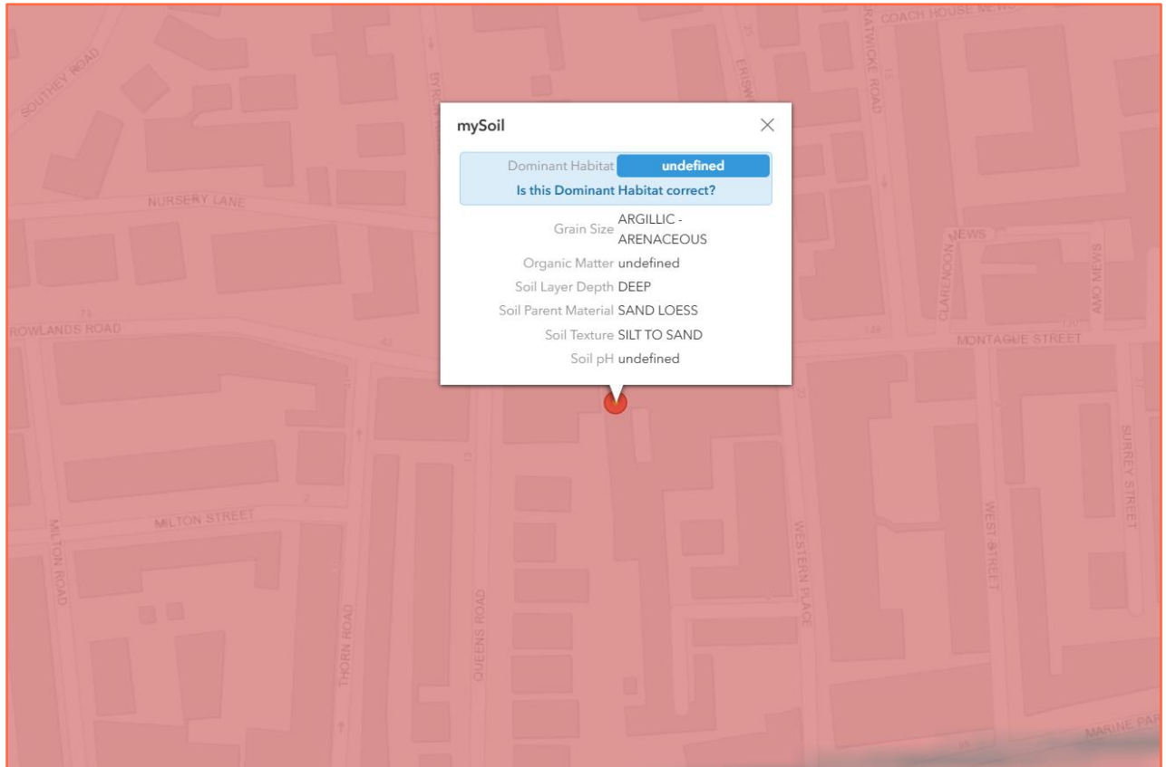
Figure 7: Soil map (Source: UK Soils, BGS)
