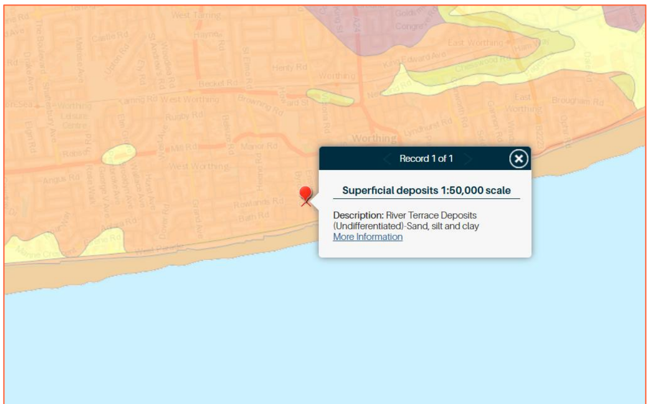
Figure 6: BGS superficial deposits (Source: BGS)
