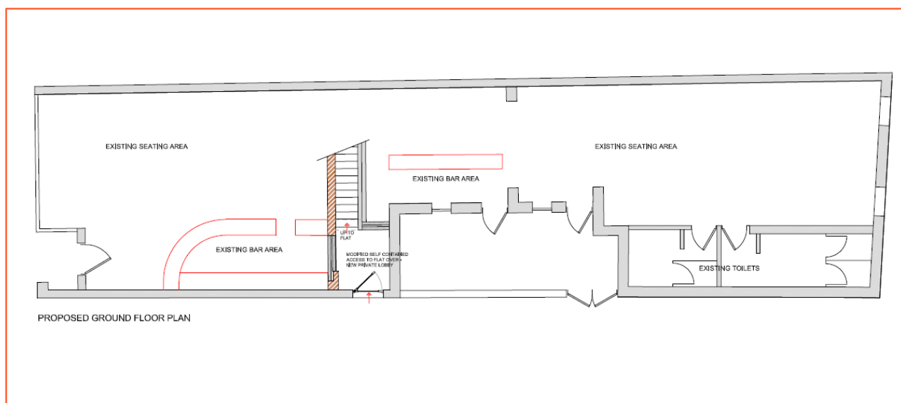
Figure 8: Proposed Ground Floor Plan (Source: Applicant)
