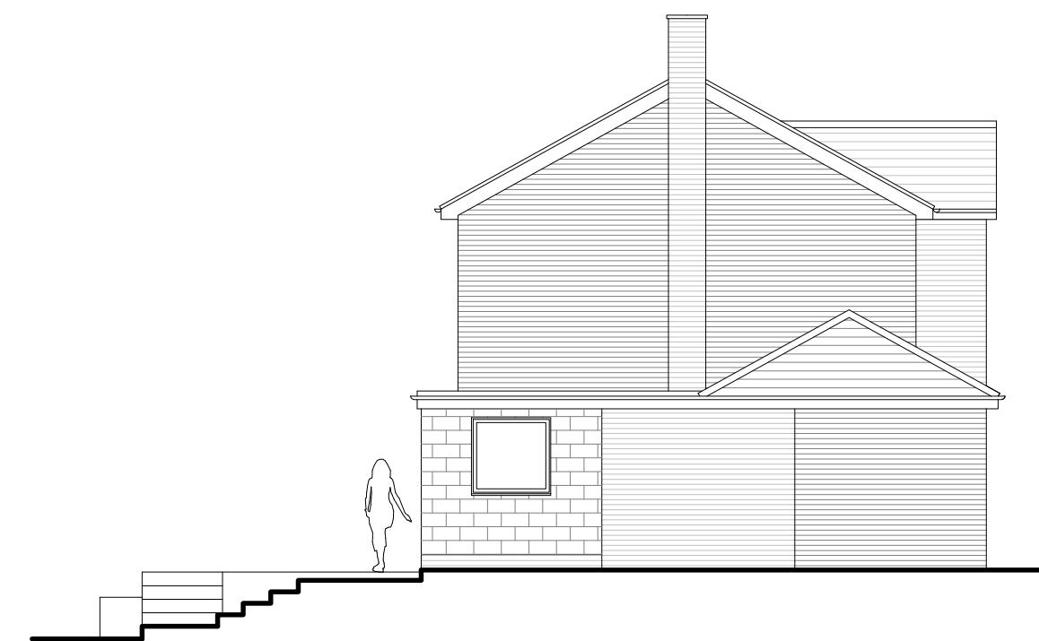
Proposed Side Elevation (South East) 1:100
