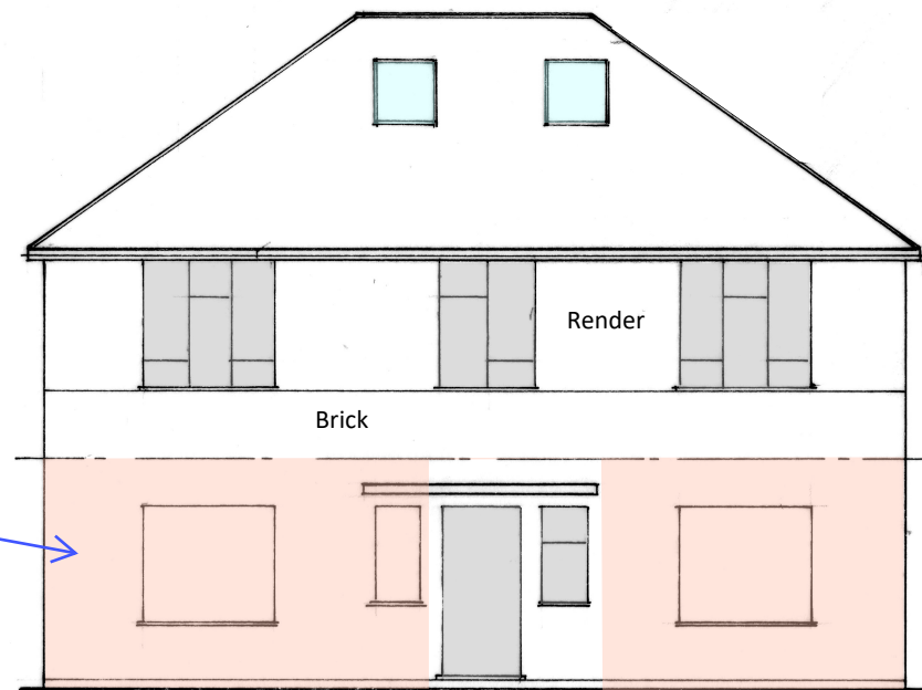
Proposed Front Elevation ( East) 1:100
