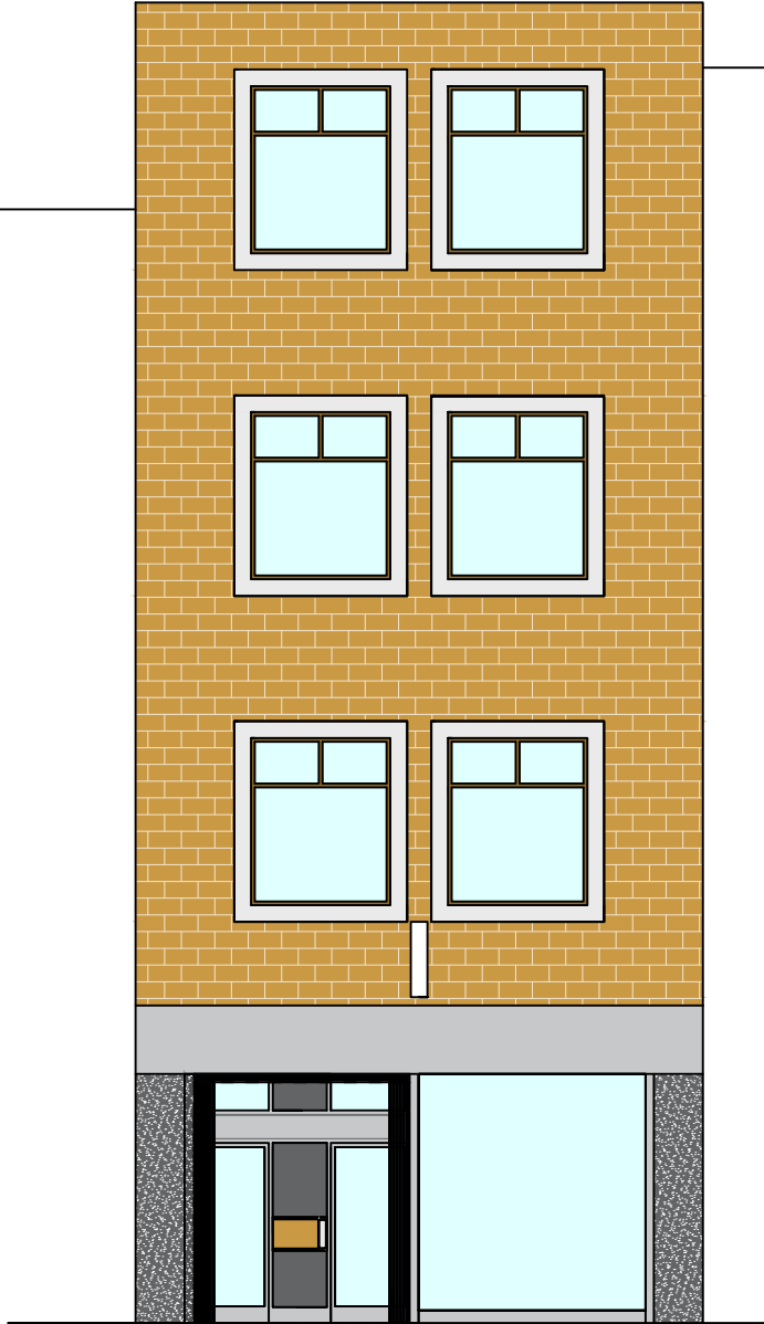
Proposed East Elevation - Grille Open
